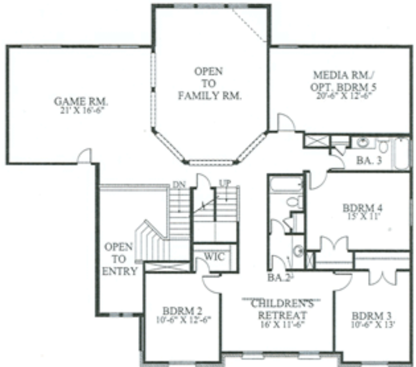
SECOND LEVEL FLOOR PLAN
