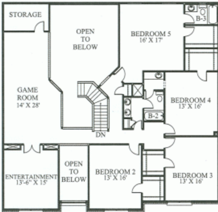
SECOND LEVEL FLOOR PLAN
