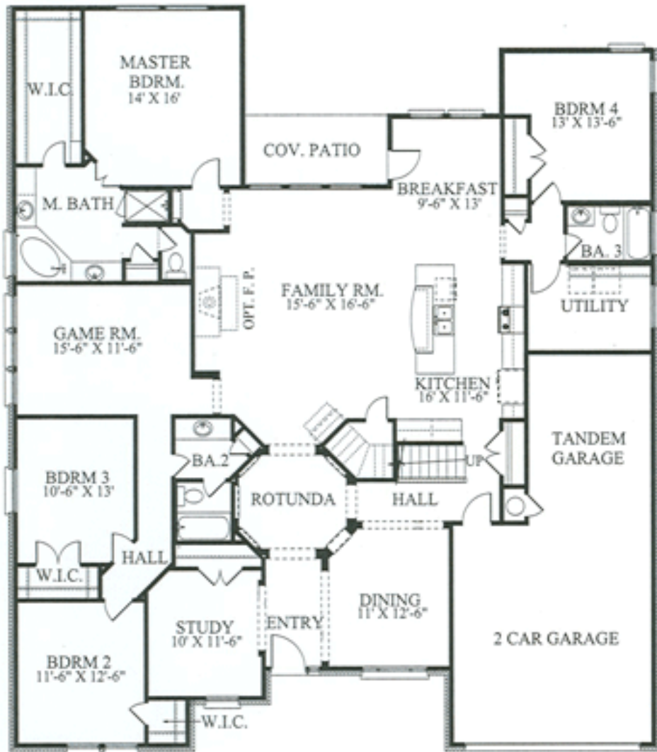
FIRST LEVEL FLOOR PLAN
